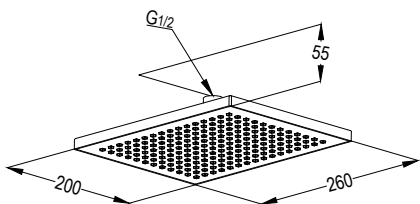
RAK22056 ABS Over head shower DN 15 260 mm x 200 mm with cleaning system with ball joint connection 1/2 inch
