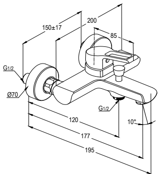
Single lever bath and shower mixer DN 15 Ceramic cartridge -K35 without shower set PCA aerator M 24 X 1 flow class CB automatic diverter shower to bathtub shower outlet G 1/2" protected against back flow S-unions 1/2 x 3/4 inch European standard - EN 817
