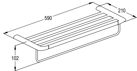
RAK20020 Towel shelf with towel bar wall fastening with screws and dowels
