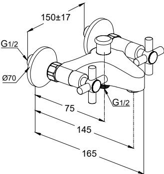
RAK34005 Dual controlled bath and shower mixer DN 15 without shower set aerator M24x1 flow class CB S-unions 1/2 inch x 3/4 inch automatic diverter : shower to bathtub shower outlet 1/2 inch European standard- EN200
