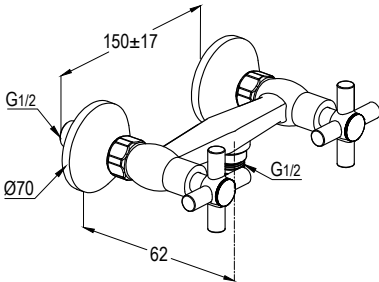
RAK34010 Dual controlled shower mixer DN 15 ceramic head part 90 ,Right & Left flow class B shower connection 1/2 inch protected against back flow S-unions 1/2 inch x 3/4 inch in accordance to EN 200
